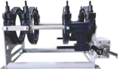
HDPE Welding Machine
